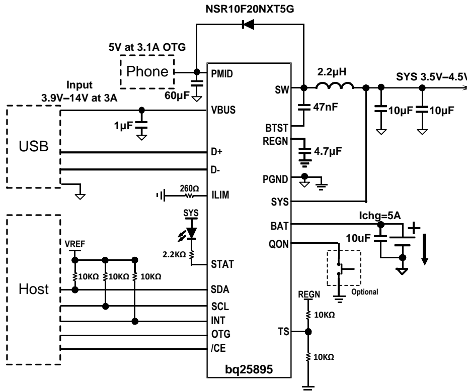
Figure 60. bq25895 with D+/D- Interface, 3.1 A Boost Mode Output, and no Thermistor Connections
