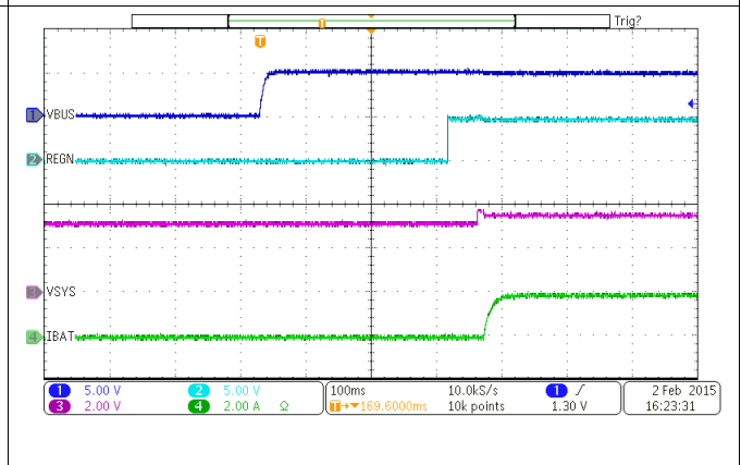
Figure 49. Power Up with Charge Disabled
