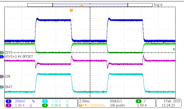
Figure 55. Load Transient During Supplement Mode
