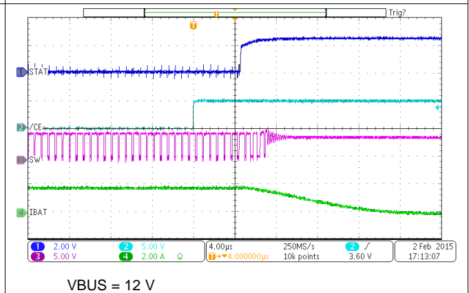
Figure 51. Power Up with Charge Enabled
