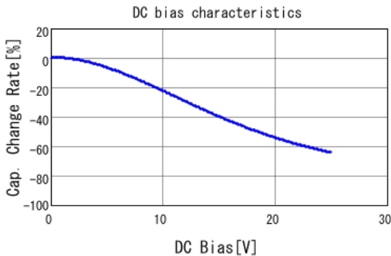
■ GRM188R71E474KA12 C-DC bias capchange, 25.0degC, AC1.
