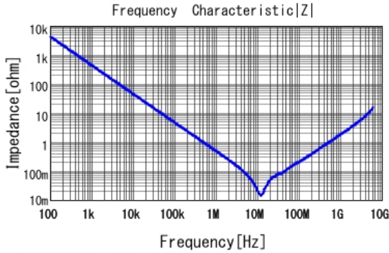
■ GRM188R71E474KA12 |Z| DCOV, 25degC
