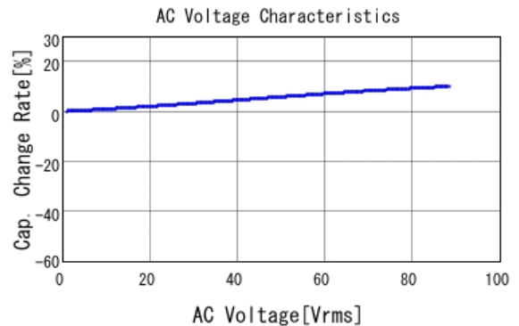
■ GRM188R72E221KW07 C-AC Voltage capchange, DCOV, 25.0d
