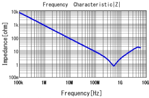
■ GRM188R72E221KW07 |Z| DCOV, 25degC
