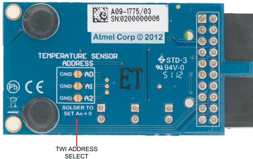
Figure 4-1 Temperature Sensor TWI Address
