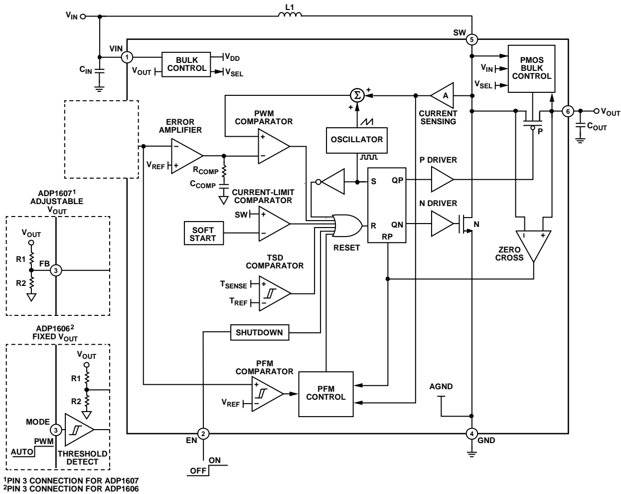
Figure 28. Block Diagram
