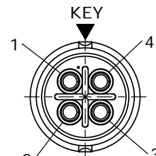
WIRING END W6380-4PG-P-3XX
