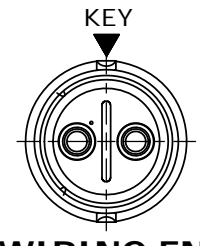
WIRING END W6380-2PG-P-3XX SHOWN WITHOUT HARDWARE
