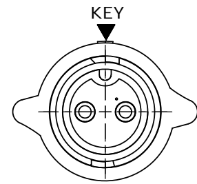
MATING FACE W6380-2PG-P-3XX SHOWN
