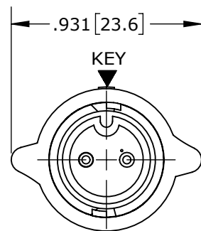
MATING FACE ASSY: W6282-2PG-P-3XX SHOWN
