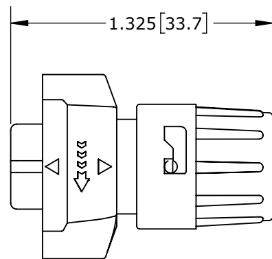
SHOWN ASSEMBLED KIT ASSY: W6282-2PG-P-3XX SHOWN
