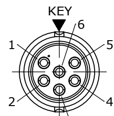
WIRING END W6282-6PG-P-3XX
