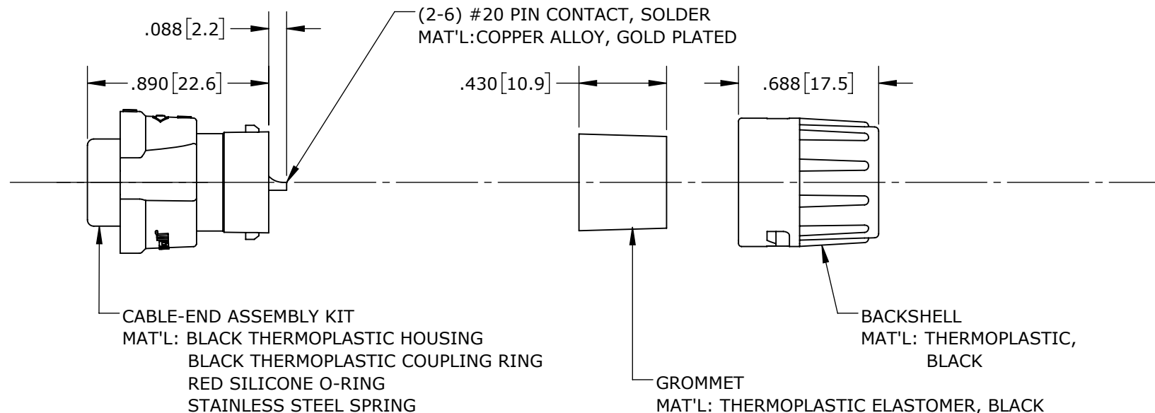
SHOWN ASSEMBLED KIT ASSY: W6282-2PG-P-3XX SHOWN
