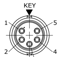
WIRING END W6282-5PG-P-3XX
