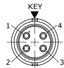
WIRING END W6282-4PG-P-3XX
