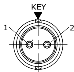
WIRING END W6282-2PG-P-3XX
