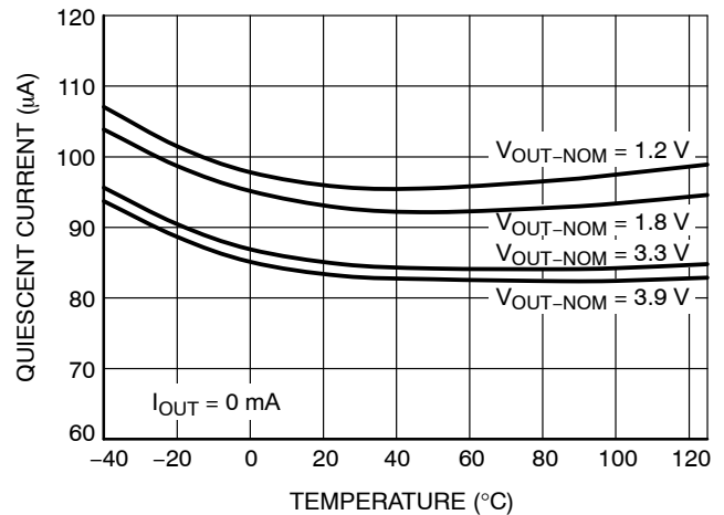
Figure 14. Quiescent Current vs. Temperature
