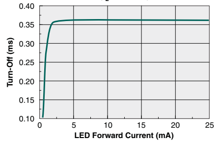
Typical Turn-Off vs. LED Forward Current (I L =120mA)
