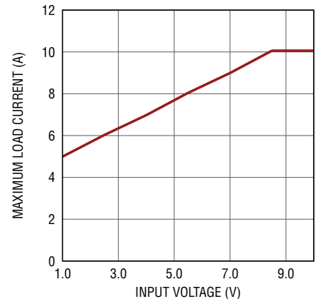
Figure 4. Load Current Derating vs Input Voltage
