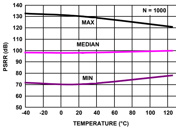
FIGURE 21. PSRR vs TEMPERATURE, V_+, V_- = \pm 0.9V \text{ TO } \pm 2.5V
