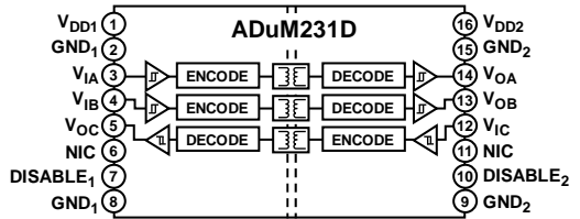
NIC = NO INTERNAL CONNECTION. LEAVE THIS PIN FLOATING. 13577-001
