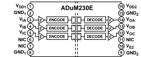
NIC = NO INTERNAL CONNECTION. LEAVE THIS PIN FLOATING. 13577-002
