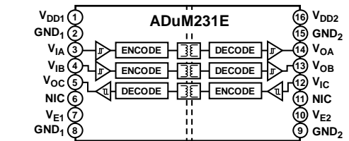
NIC = NO INTERNAL CONNECTION. LEAVE THIS PIN FLOATING. 13577-102
