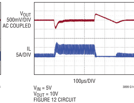
Load Step (Boost) Pulse-Skipping Mode
