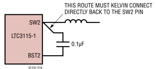
Figure 15. Kelvin BST Connections
