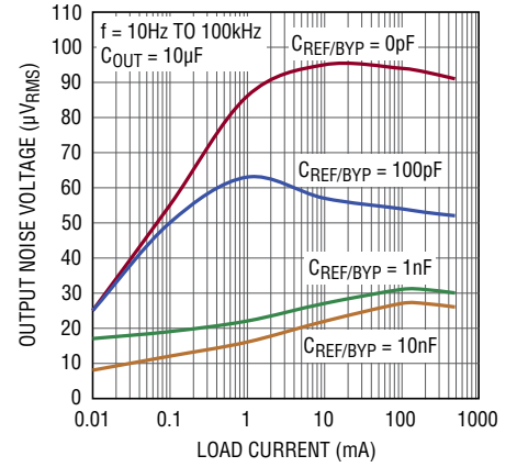
RMS Output Noise, V_{\text{OUT}} = 0.6\text{V} , C_{\text{FF}} = 0
