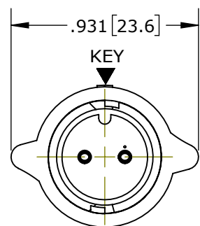
MATING FACE ASSY: W6282-2SG-P-3XX SHOWN
