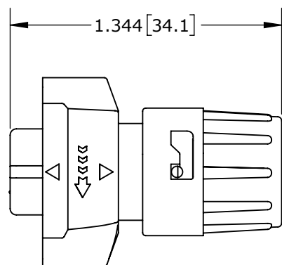
SHOWN ASSEMBLED KIT ASSY: W6282-2SG-P-3XX SHOWN
