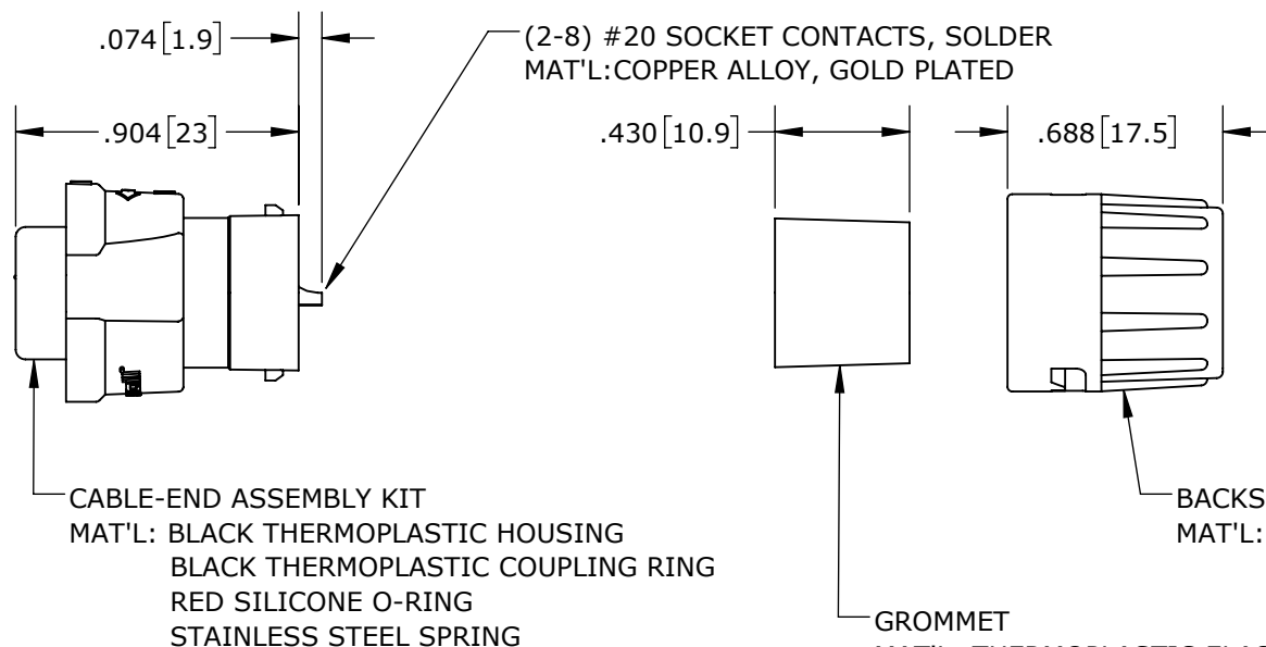
SHOWN ASSEMBLED KIT ASSY: W6282-2SG-P-3XX SHOWN
