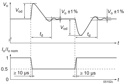
Fig. 4 Typical dynamic load regulation of output voltage
