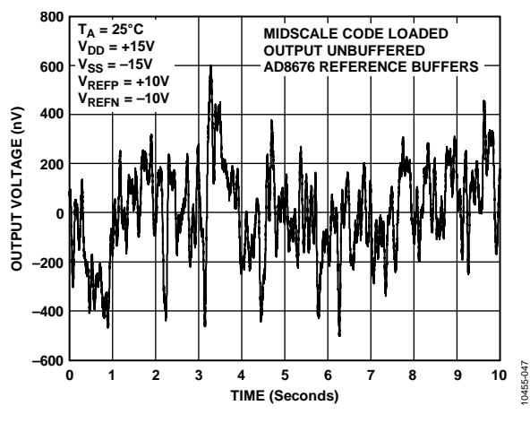
Figure 46. Voltage Output Noise, 0.1 Hz to 10 Hz Bandwidth
