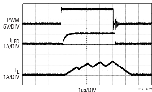
2000:1 PWM Dimming at 120Hz
