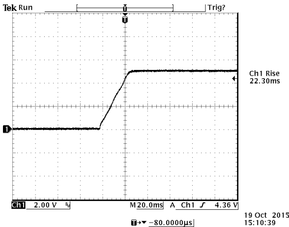
Figure 17. V_{in} = 48\text{ V} , I_o = 6\text{ A} , V_o = 5\text{ V} , with C_{ext} = 1000\ \mu\text{F}
