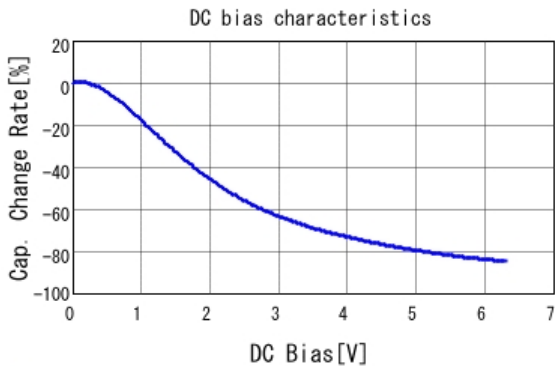
■ GRM155R60J106ME47 C-DC bias capchange, 25.0degC, ACO.
