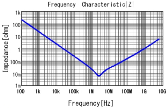
■ GRM155R60J106ME47 |Z| DCOV, 25degC
