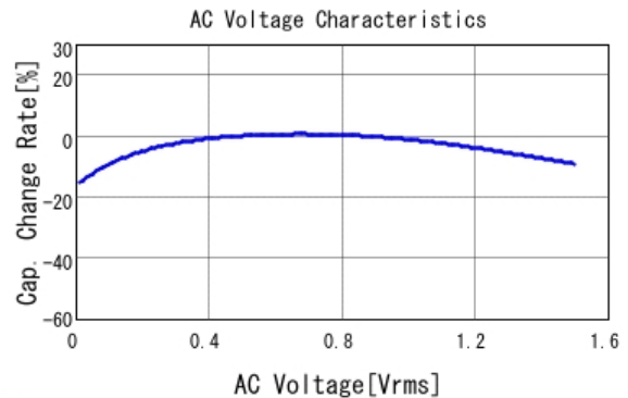
■ GRM155R60J106ME47 C-AC Voltage capchange, DCOV, 25.0d
