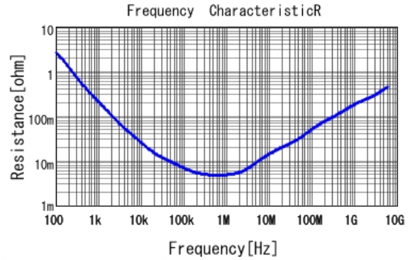
■ GRM155R60J106ME47 R DCOV, 25degC
