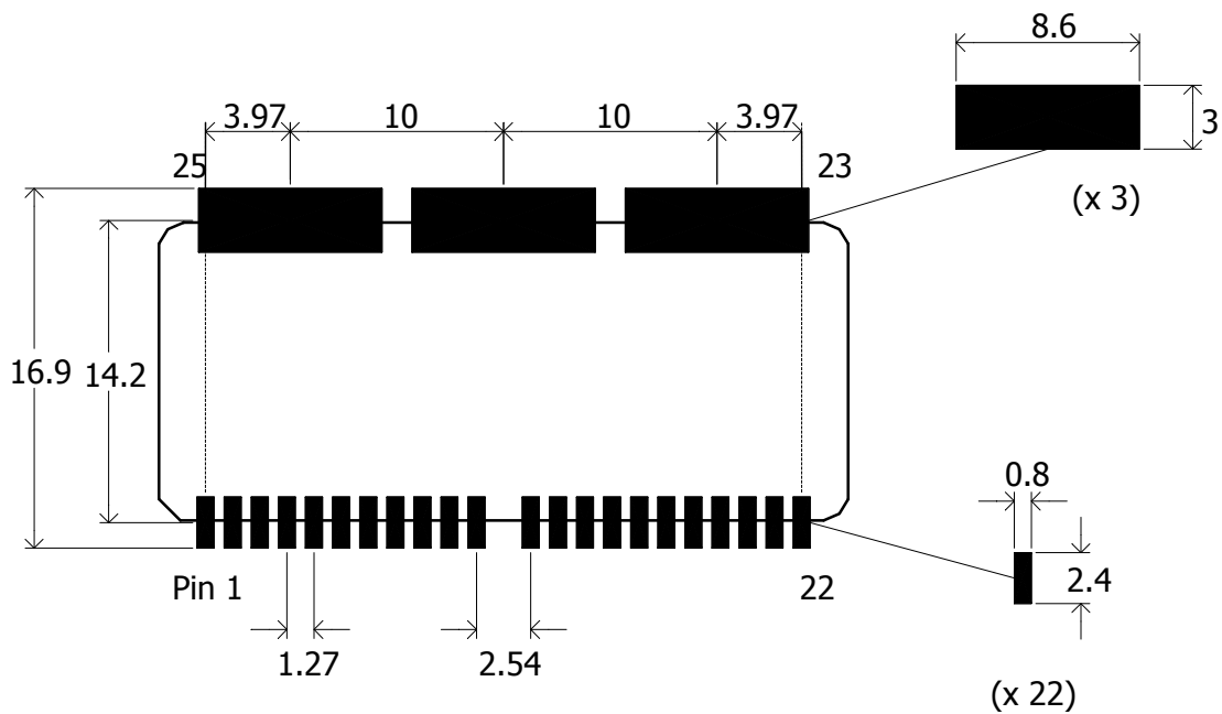
Figure 49. Recommended Pad Sizes
