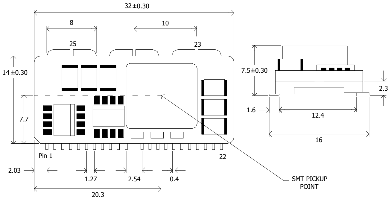
Figure 48. Mechanical Drawing
