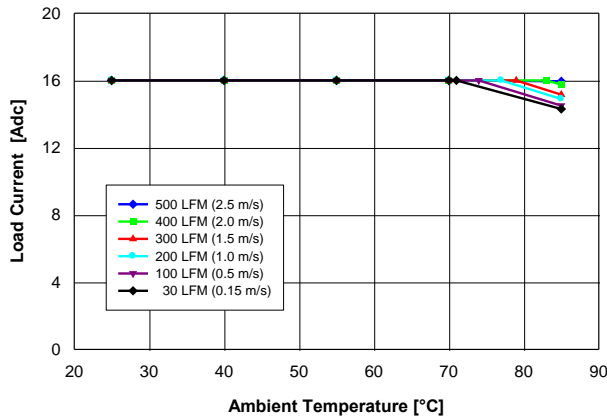
Fig. 1.5V.1: Available load current vs. ambient temperature and airflow rates for V_{out} = 1.5V converter mounted vertically with V_{in} = 12V , air flowing and maximum MOSFET temperature \leq 120^\circ C .
