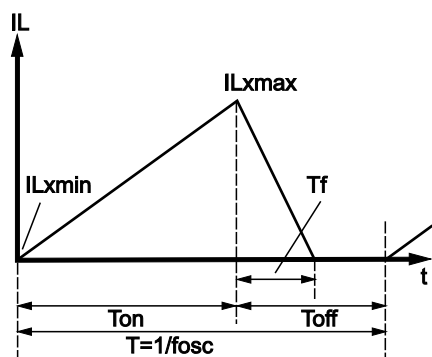
Discontinuous Mode
