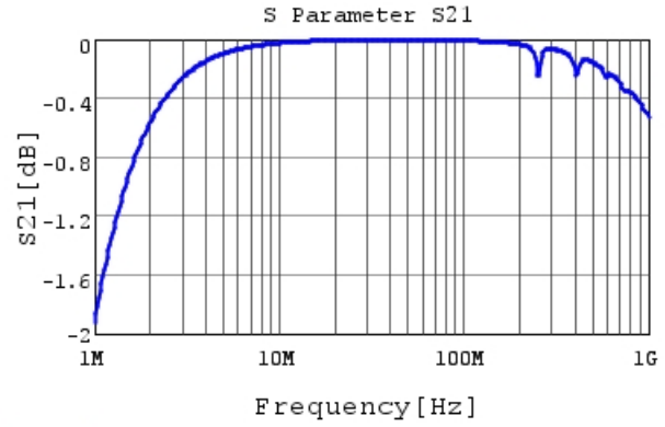
RDE7U3A222J3K1H03B S21 DCOV, 25degC
