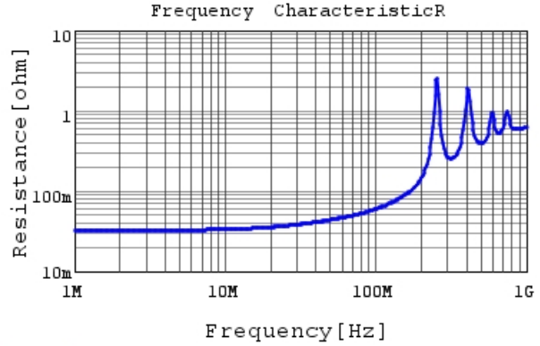
RDE7U3A222J3K1H03B R DC0V, 25degC
