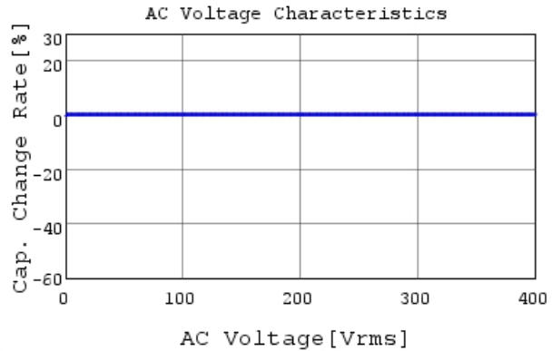
RDE7U3A222J3K1H03B C-AC Voltage capchange, I
