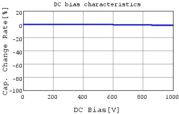
RDE7U3A222J3K1H03B C-DC bias capchange, 25.0
