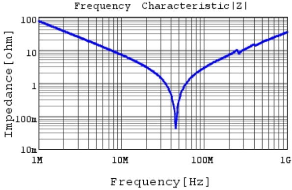
RDE7U3A222J3K1H03B |Z| DC0V, 25degC
