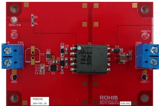
Figure 1. BD7F100HFN-EVK-002 Evaluation Board
