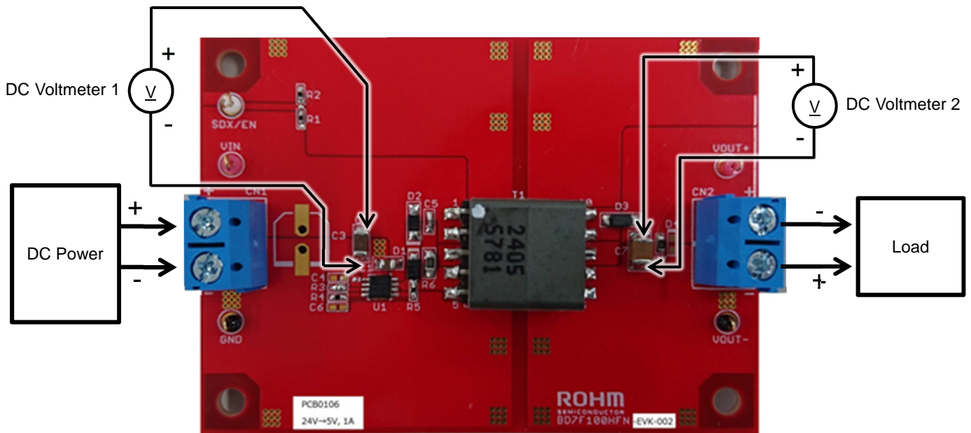
Figure 3. Connection Diagram
