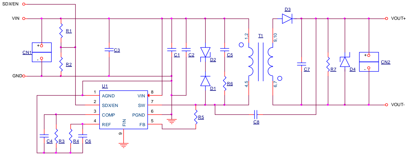
Figure 4. BD7F100HFN-EVK-002 Circuit Diagram
