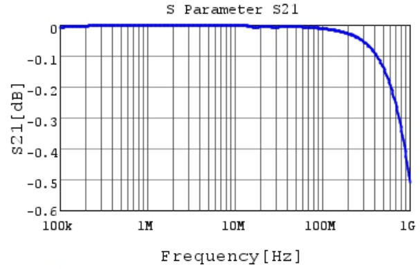
RDED72W474K5B1H03B S21 DCOV, 25degC
