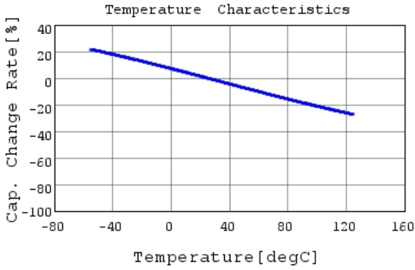
RDED72W474K5B1H03B C-Temp. capchange, DCOV,
