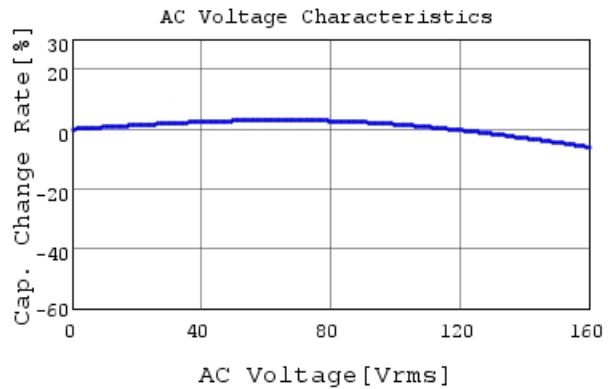
RDED72W474K5B1H03B C-AC Voltage capchange, I
