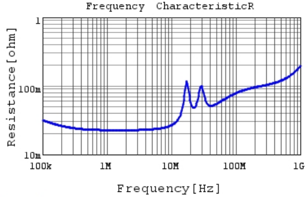
RDED72W474K5B1H03B R DC0V, 25degC
