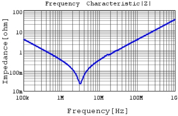
RDED72W474K5B1H03B |Z| DC0V, 25degC
