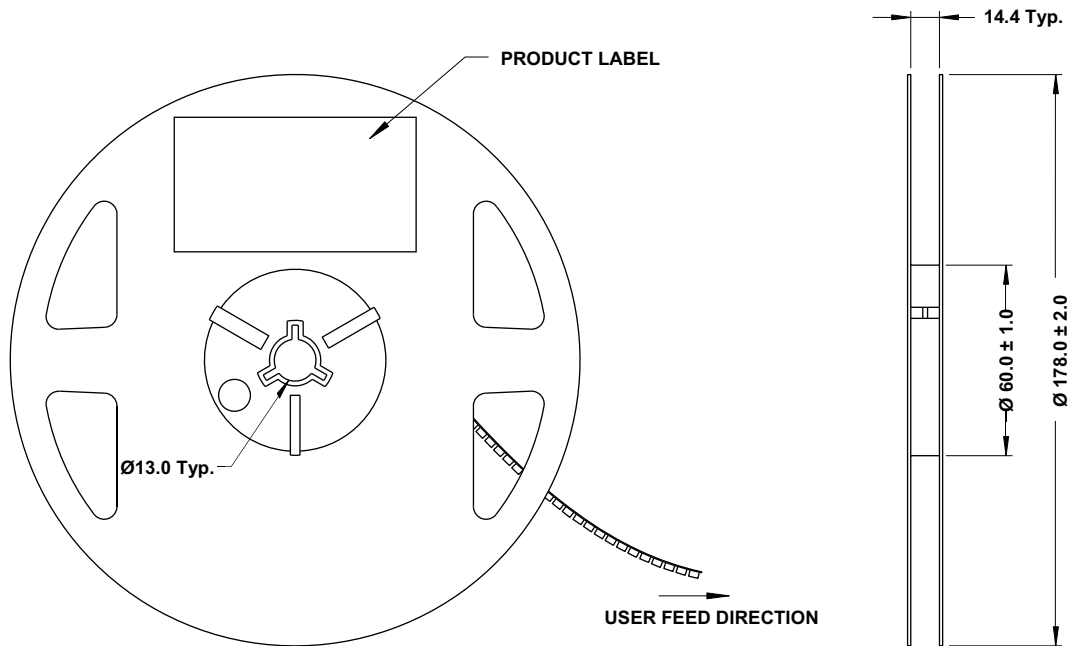
Figure 15: Reel Dimensions
