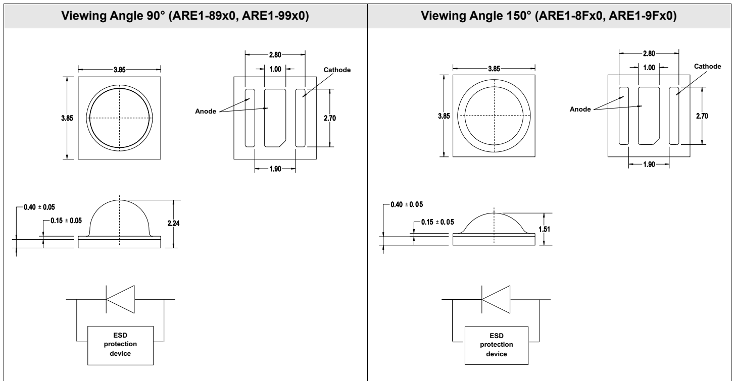
Figure 1: Package Drawing
