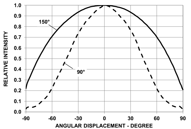
Figure 7: Radiation Pattern
