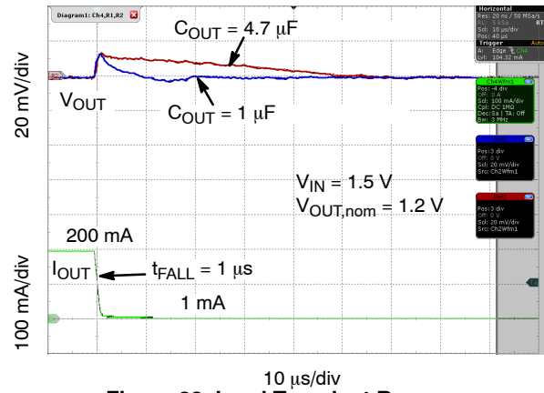
Figure 32. Load Transient Response, I_{OUT} = 1 \text{ mA} to 200 \text{ mA}
