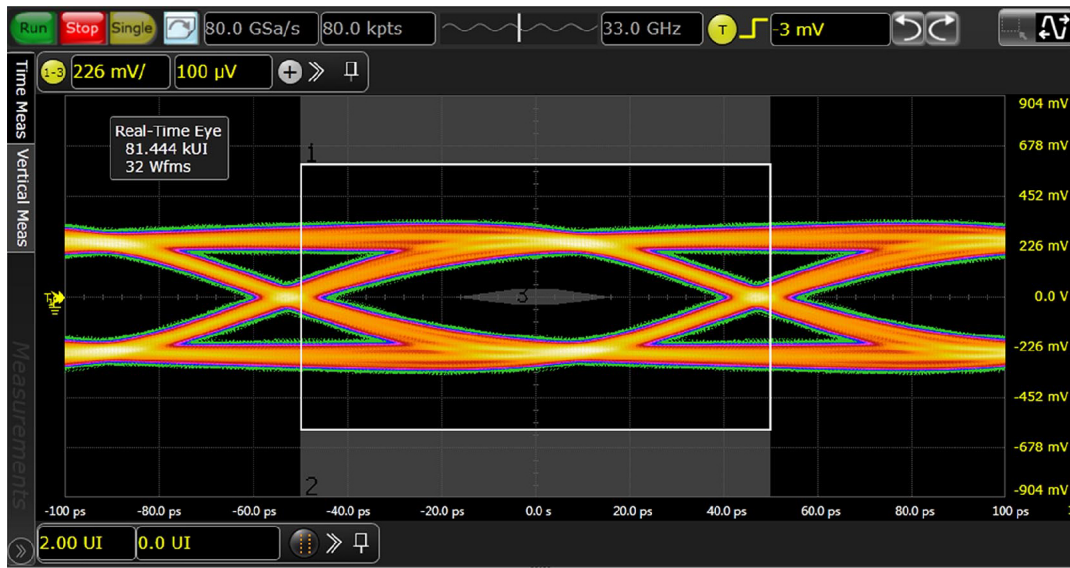
Fig. 5. USB3.2 eye diagram 10 Gbps, PCB with device; typical values
