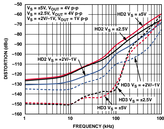
Figure 16. Distortion vs. Frequency, G = +2
