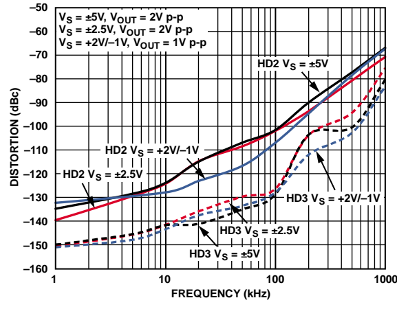
Figure 15. Distortion vs. Frequency for Various Supplies, G = +1
