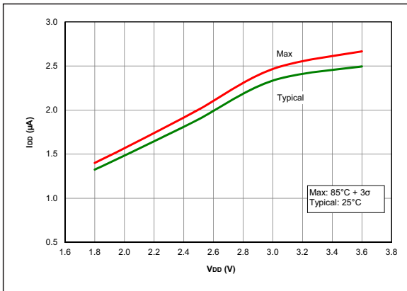
FIGURE 36-3: I_{DD} , HS Oscillator, 32 MHz, PIC16LF18324/18344 Only
