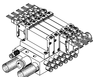
Valve manifold assembly VTUG comprising sub-base valves VUVG-BK/VUVG-B
