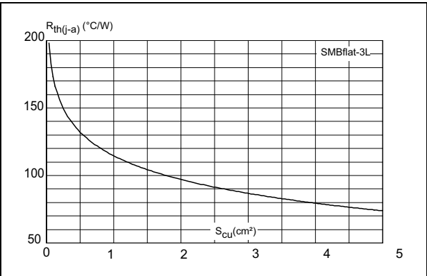
Figure 6. Typical thermal resistance junction to ambient versus copper surface under anode (epoxy FR4, Cu_{th} = 35 \mu m )
