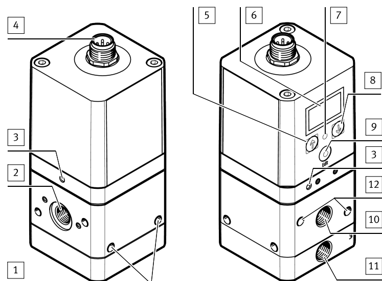
Fig. 2 Product design VPPE-...-E1
