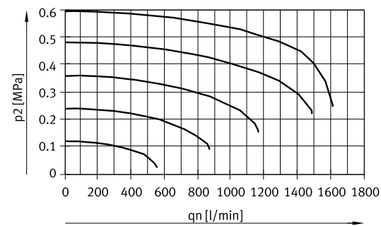
Fig. 6 VPPE-3-1-1/8-6-... p1 = 0.8 MPa
