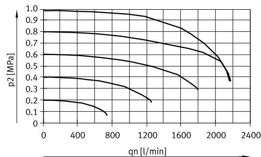
Fig. 7 VPPE-3-1-1/8-10-... p1 = 1.1 MPa
