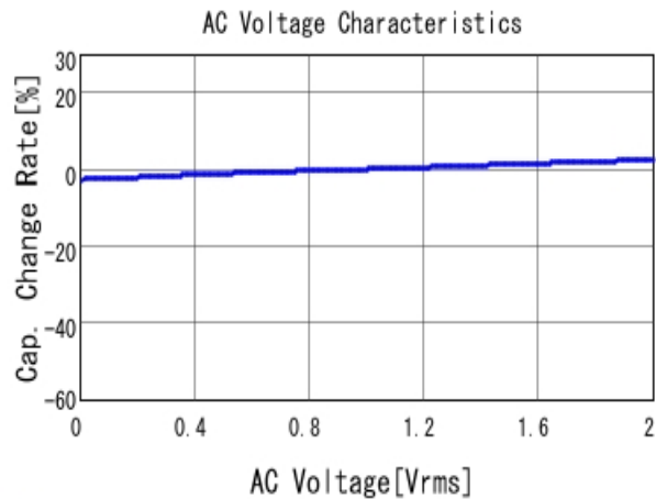
GCM188L81H104KA57 C-AC Voltage capchange, DC0V, 25.0d
