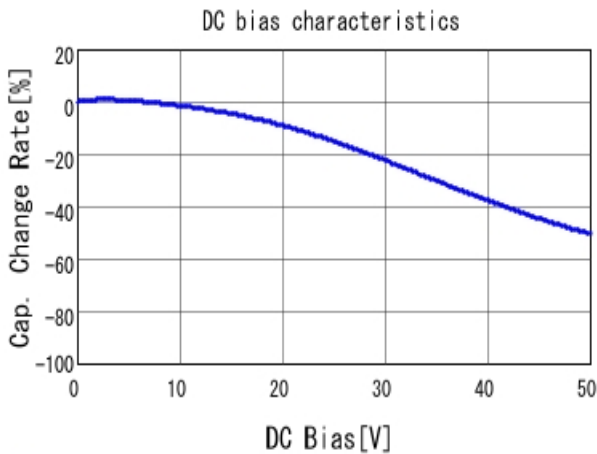
GCM188L81H104KA57 C-DC bias capchange, 25.0degC, AC1.
