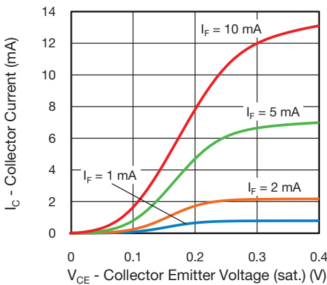
Fig. 3 - Collector Current vs. Collector Emitter Voltage (saturated)
