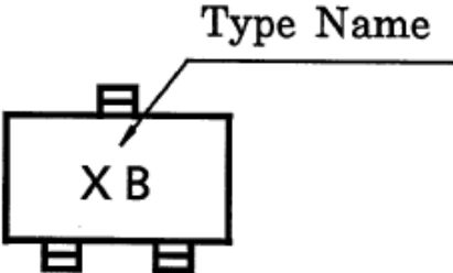
Fig. 9.2 Marking RN1402
