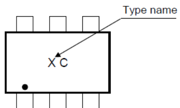
Fig. 9.3 Marking RN1903FE
