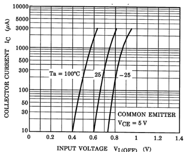
Fig. 10.12 RN1906FE I_C - V_{I(\text{OFF})}
