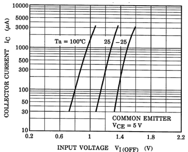
Fig. 10.8 RN1902FE I_C - V_{I(\text{OFF})}
