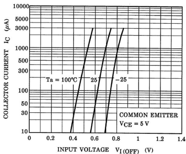
Fig. 10.11 RN1905FE I_C - V_{I(\text{OFF})}
