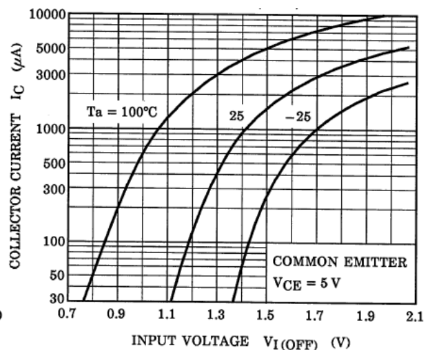
Fig. 10.10 RN1904FE I_C - V_{I(\text{OFF})}
