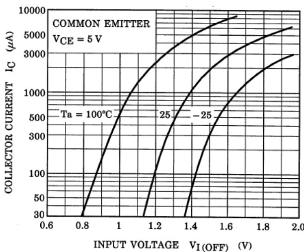
Fig. 10.9 RN1903FE I_C - V_{I(\text{OFF})}
