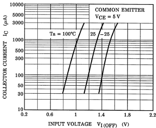
Fig. 10.7 RN1901FE I_C - V_{I(\text{OFF})}
