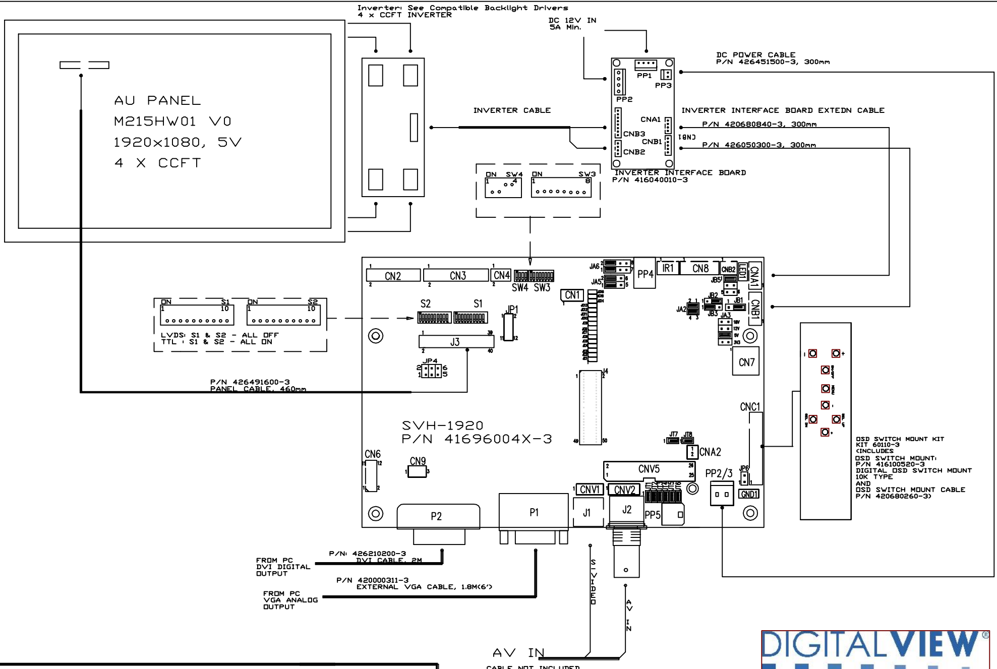
CONNECTION DIAGRAM: (PRELIMINARY) SVH-1920 FOR AU M215HW01 V0 1920x1080
