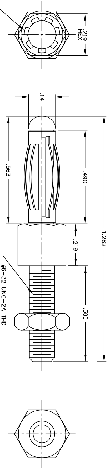
FULL SECTION VIEW
