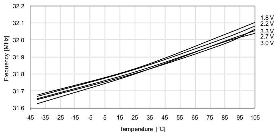
Figure 33-202. 32MHz Internal Oscillator Frequency vs. Temperature DPLL enabled, from the 32.768kHz internal oscillator
