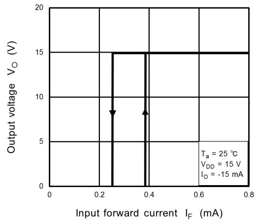
Fig. 12.2.4 V_O - I_F(IHYS)
