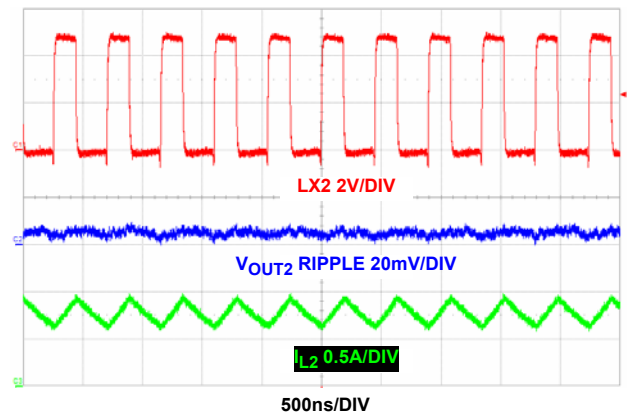
FIGURE 20. STEADY STATE OPERATION WITH FULL LOAD CHANNEL 2
