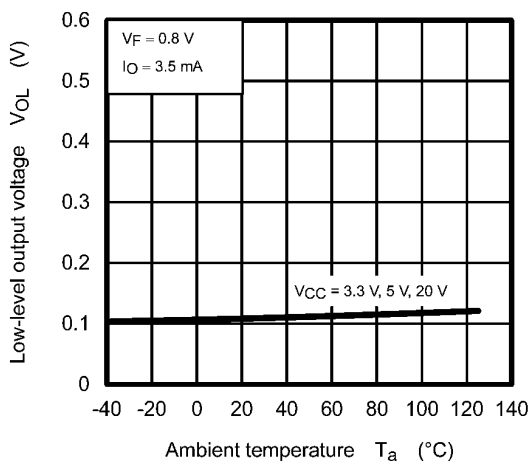
Fig. 12.2.3 V_{OL} - T_a
