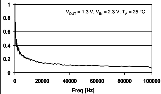
Figure 28. LD39115J noise
