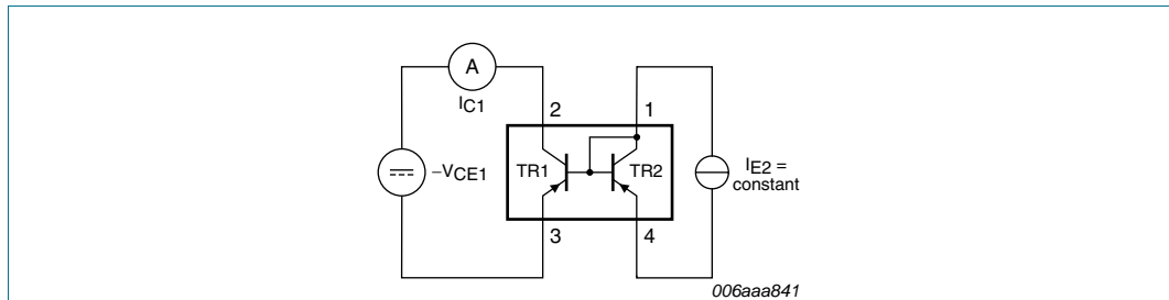
Fig 14. Test circuit current matching
