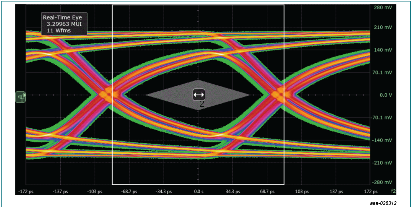
Fig. 10. Universal Flash Storage (UFS) eye diagram, PCB with device; typical values
