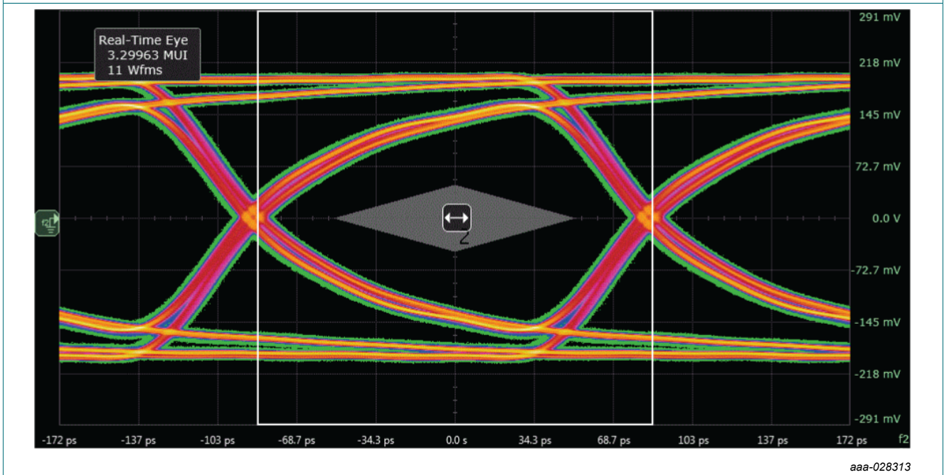
Fig. 11. Universal Flash Storage (UFS) eye diagram, PCB without device; typical values
