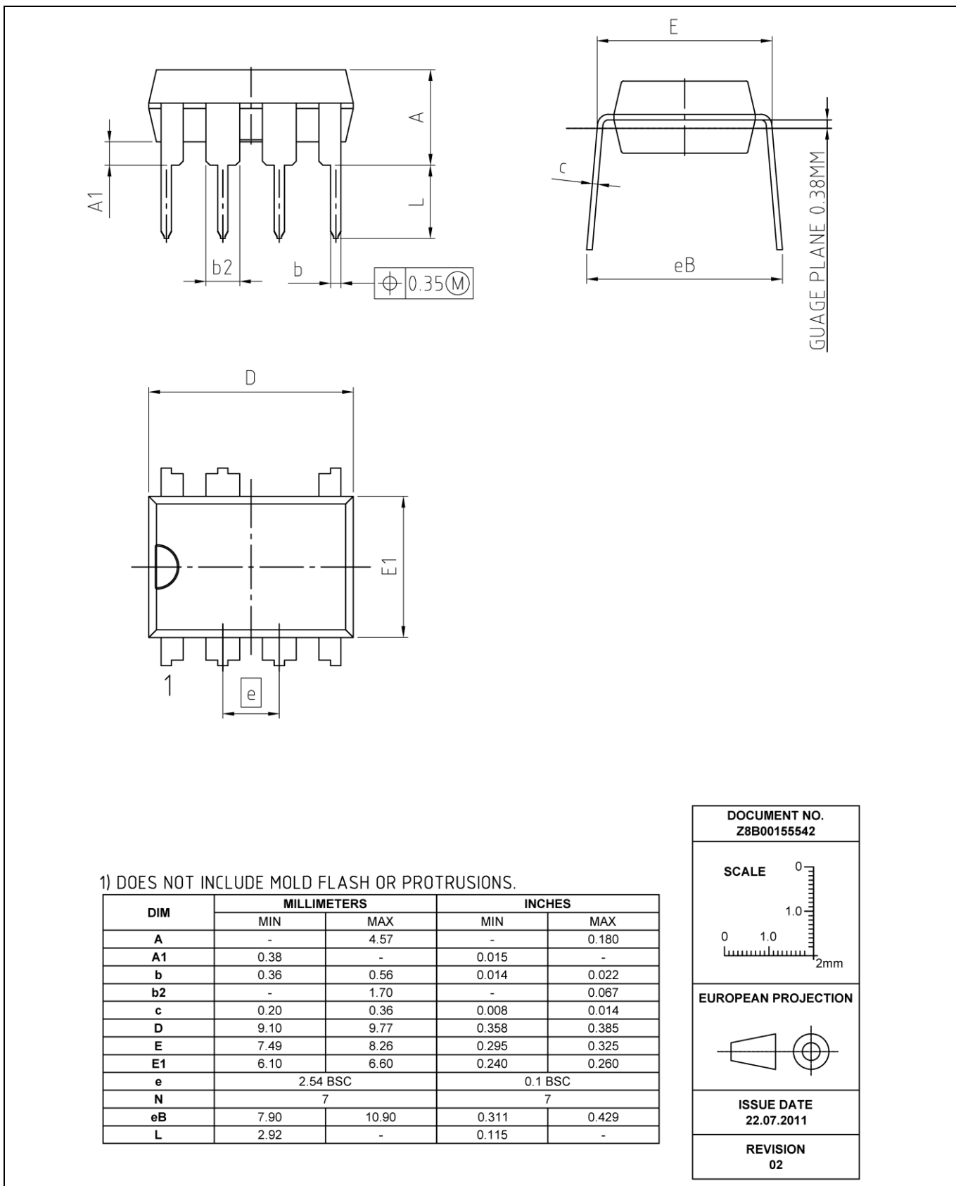
Figure 59 PG-DIP-7
