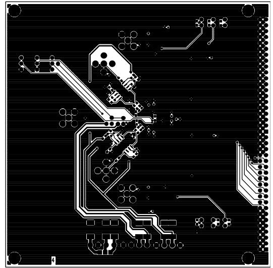
Figure 32. Bottom Routing
